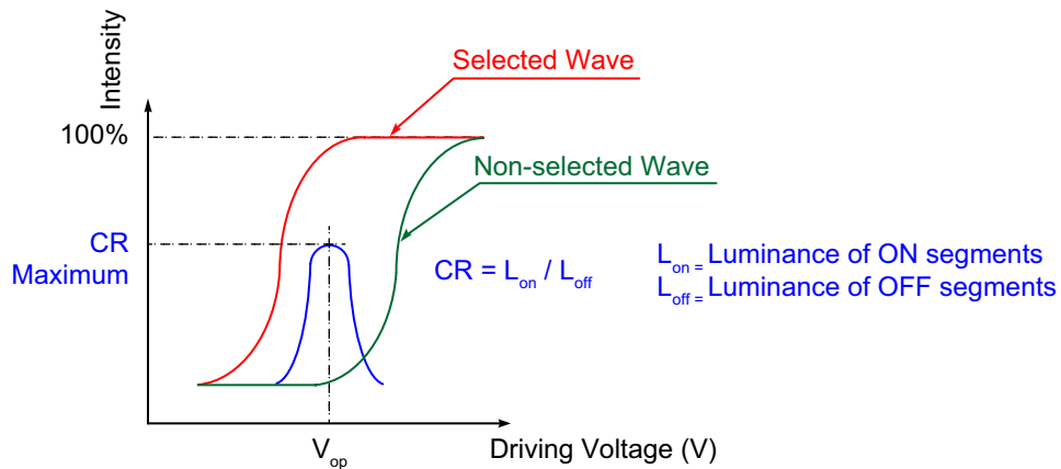
Figure 6. Definition of Operation Voltage (V OP )
