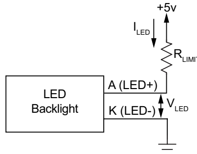
Figure 10. Typical LED Backlight Connections for “Always On”
