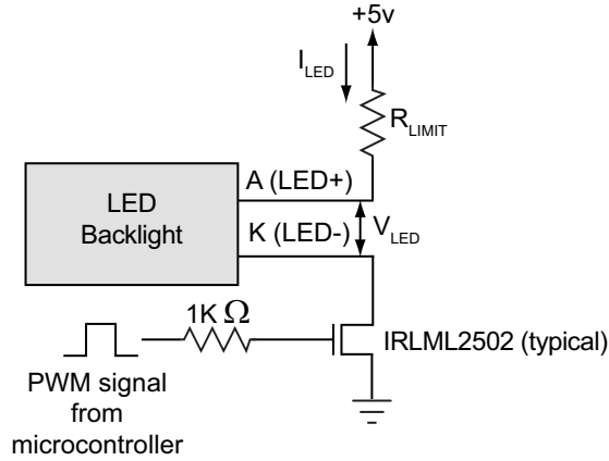
Figure 11. Typical LED Backlight Connections for PWM Dimming
