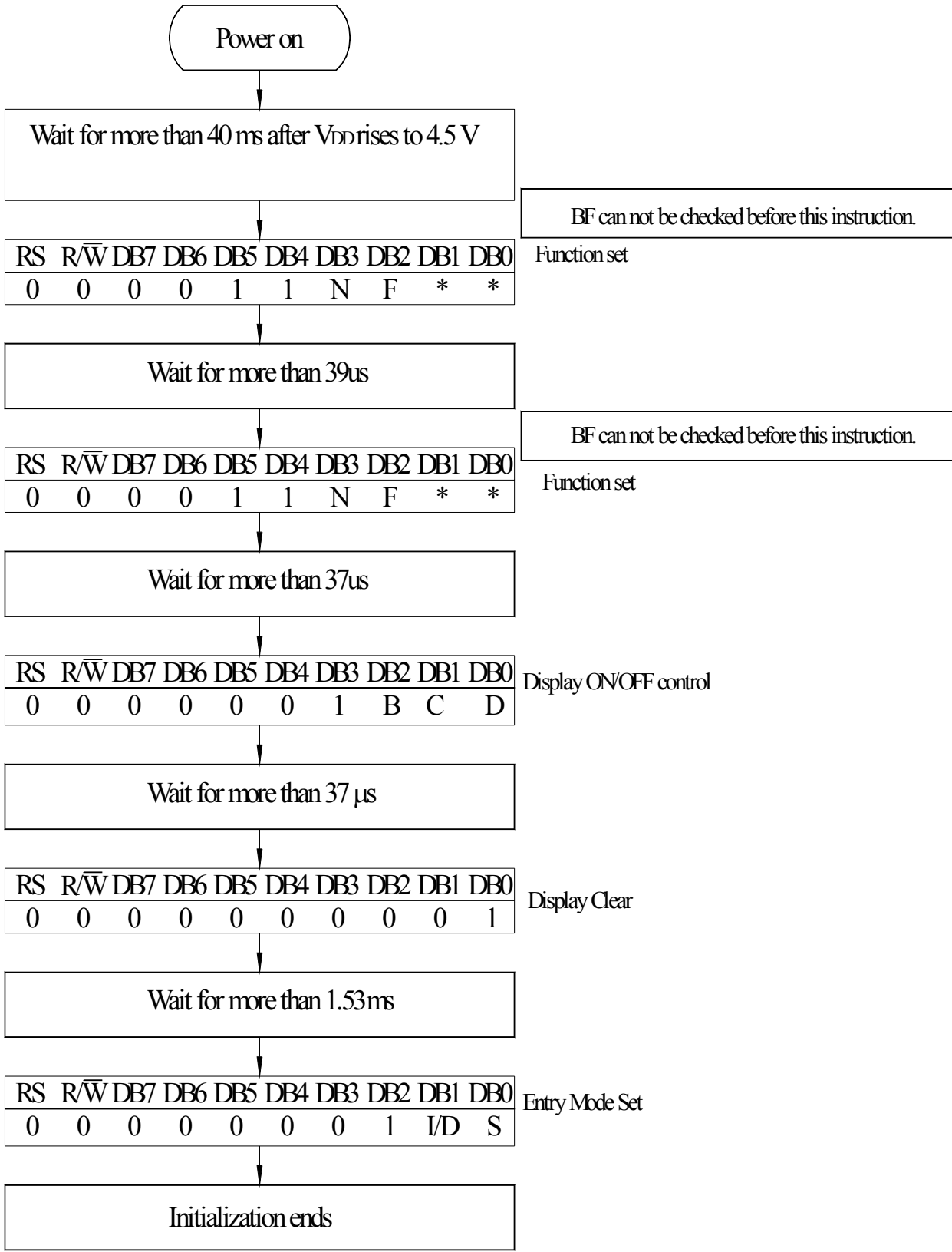
8-Bit Ineterface
