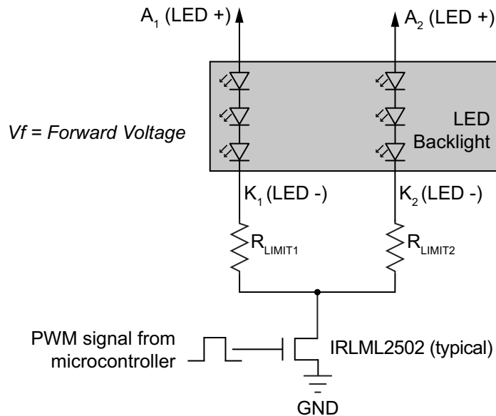
Figure 8. Example of LED Backlight Connections for PWM Dimming
