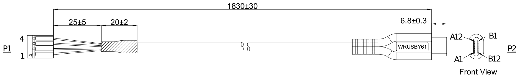
Wiring Diagram
