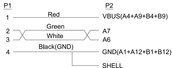
Wiring Diagram
