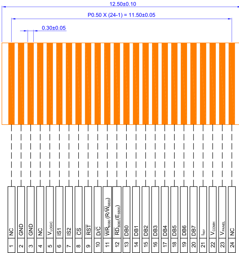
(A) Contact Side Detail
