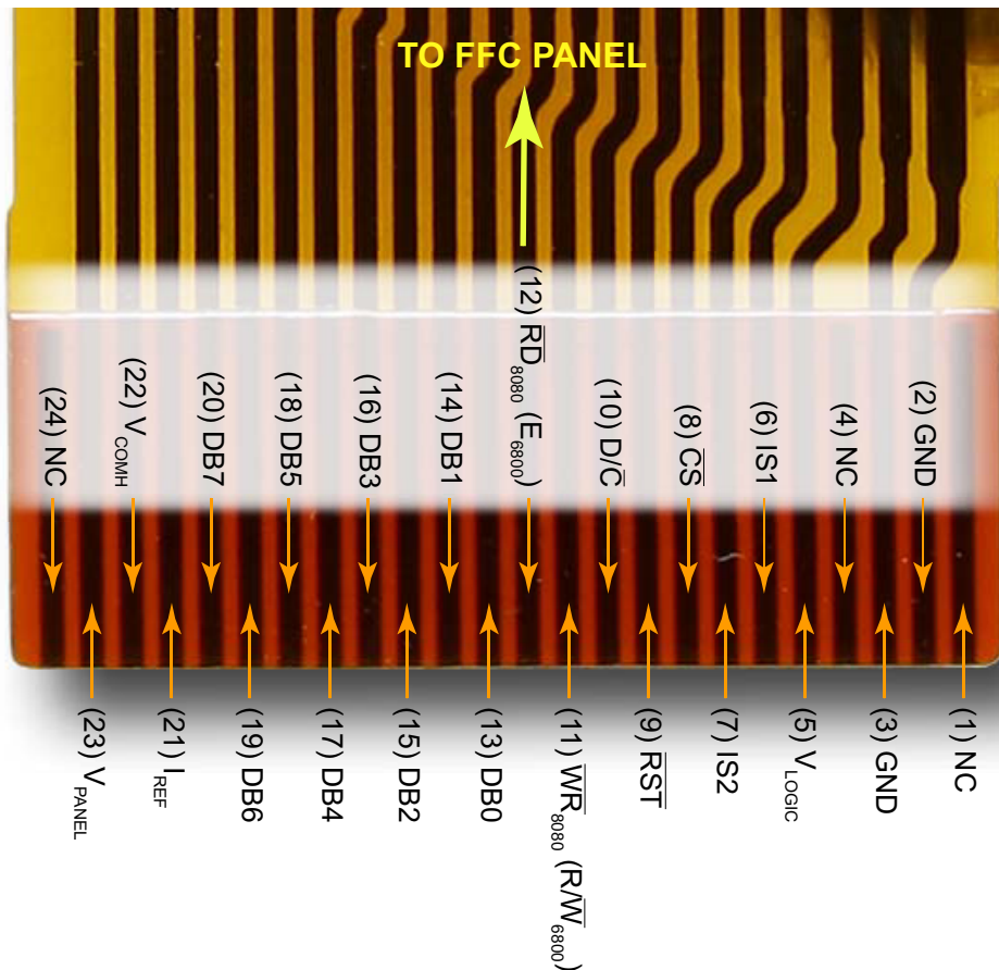
Figure 5. Back View of ZIF Connector Pins (Labeled)
