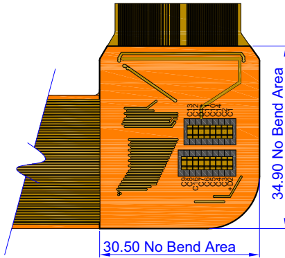
No Bend Area Detail A
