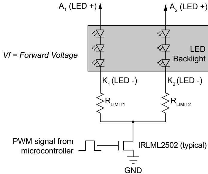
Figure 8. Example of LED Backlight Connections for PWM Dimming
