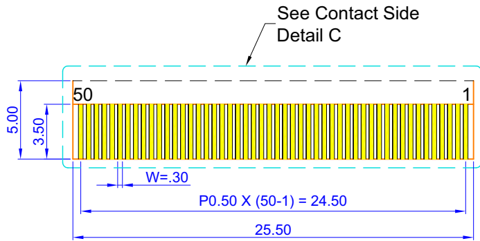
Contact Side Detail A
