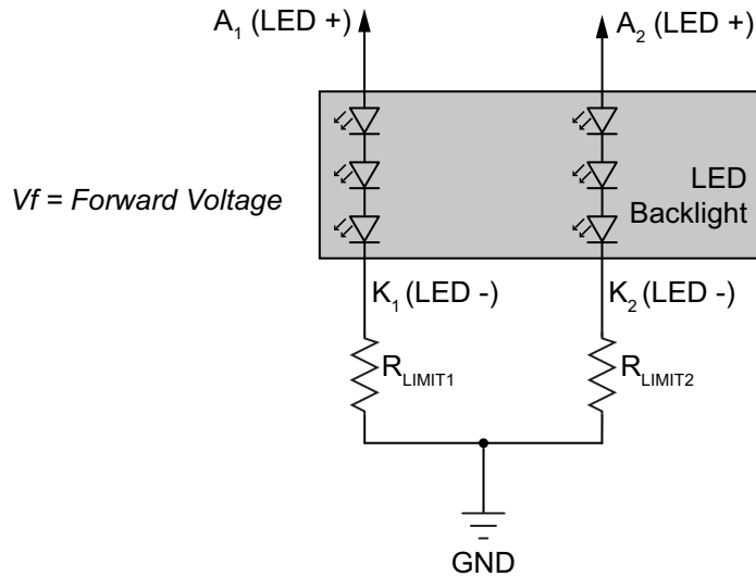
Figure 7. Typical LED Backlight Connections for "Always On"
