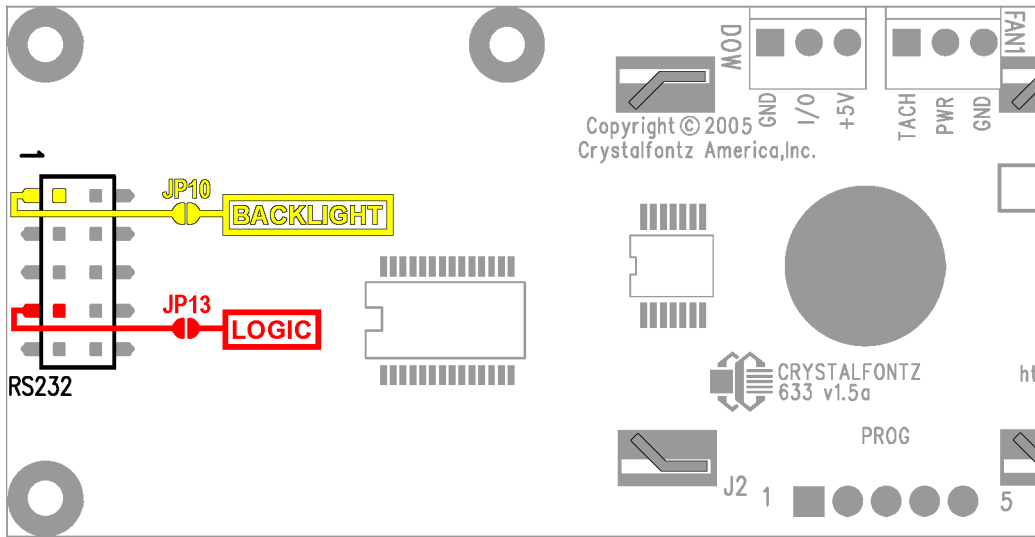
Figure 3. CFA633-RMC-KS RS-232 power connection
