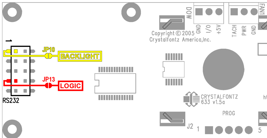
Figure 3. CFA633-RMC-KS RS-232 power connection
