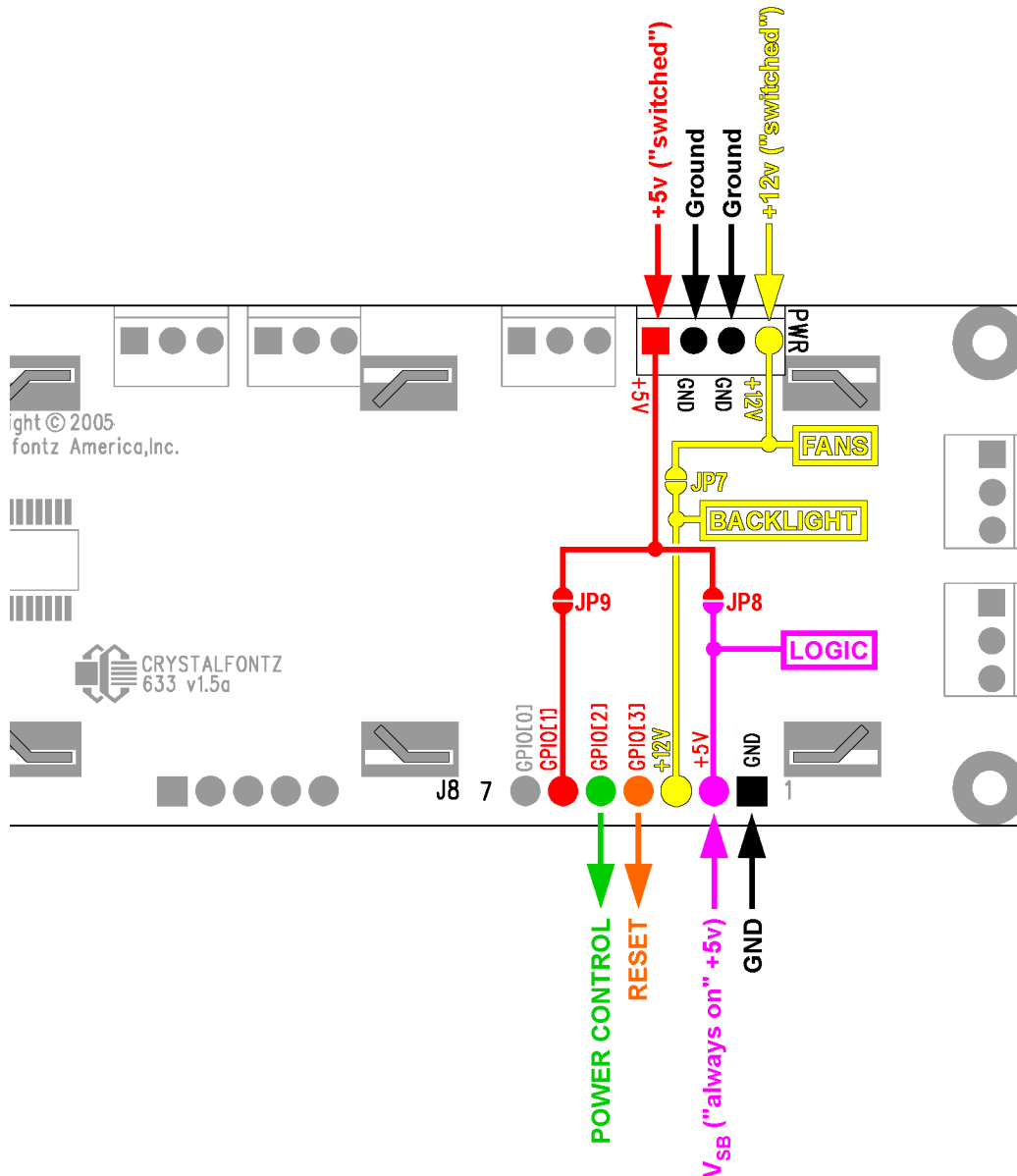
Figure 4. CFA633-RMC-KS ATX power supply and control connections
