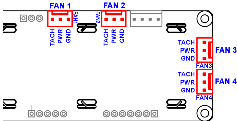
Figure 6. CFA633-RMC-KS's four fan connections
