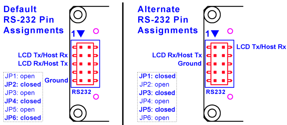
Figure 5. CFA633-RMC-KS default and alternate pin assignments
