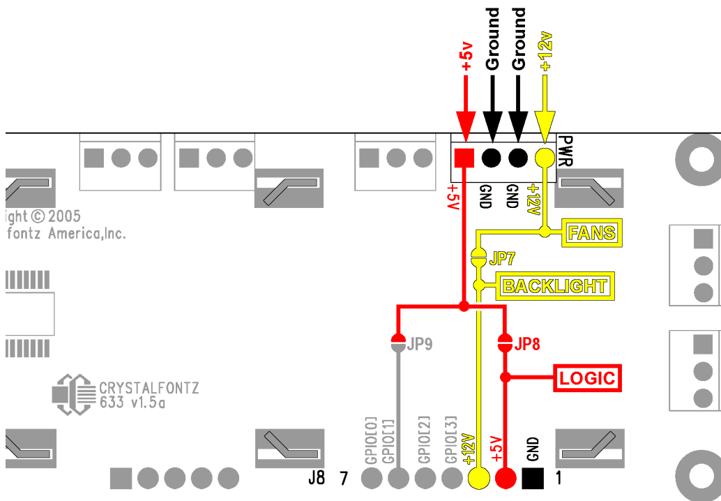
Figure 2. CFA633-RMC-KS connection for standard "3 1/2 inch floppy" power supply cable
