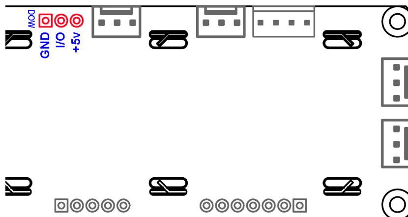
Figure 8. CFA633-RMC-KS connection for Dallas Semiconductor 1-wire (DOW) devices
