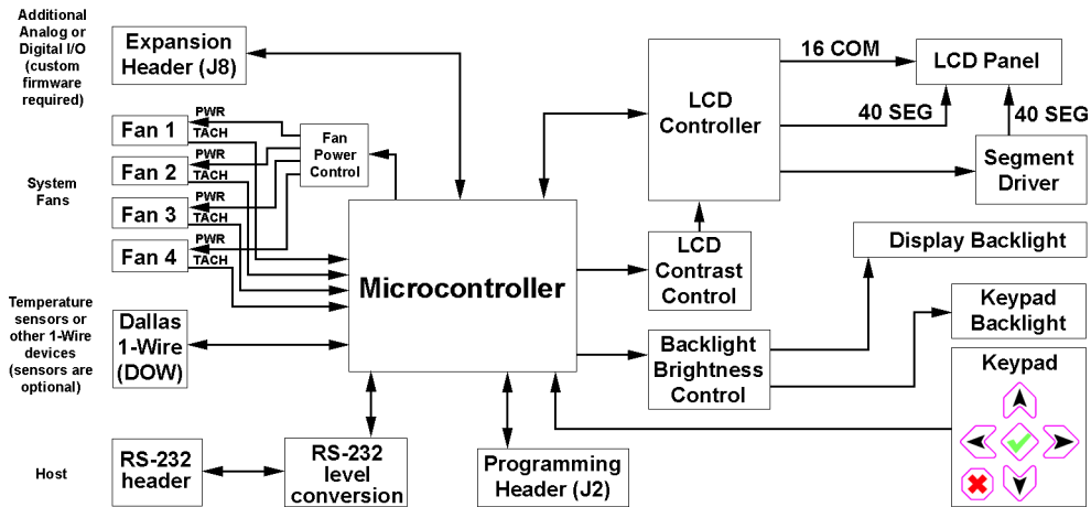
Figure 1. CFA-633 System Block Diagram
