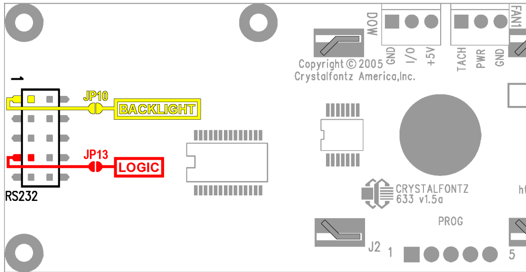
Figure 3. CFA-633 RS-232 power connection
