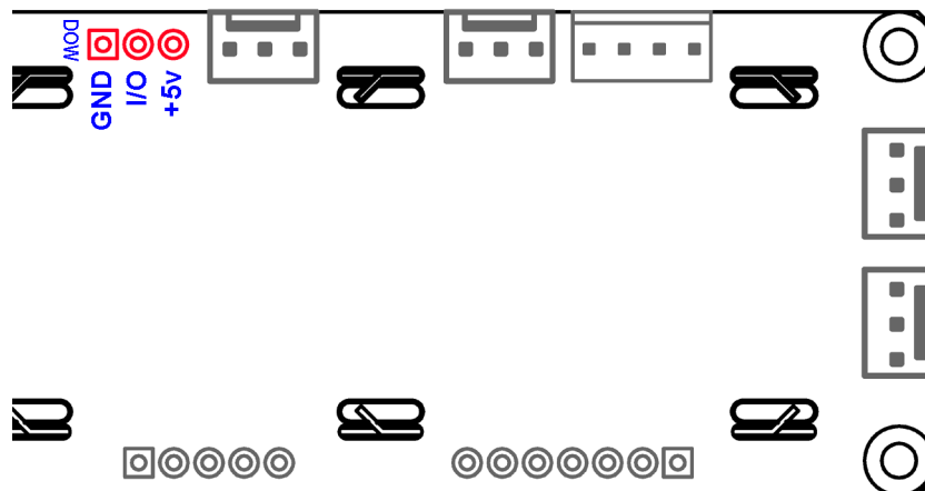
Figure 8. CFA-633 connection for Dallas Semiconductor 1-wire (DOW) devices
