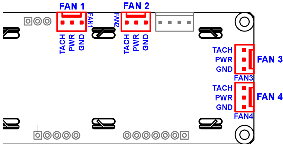
Figure 6. CFA-633's four fan connections
