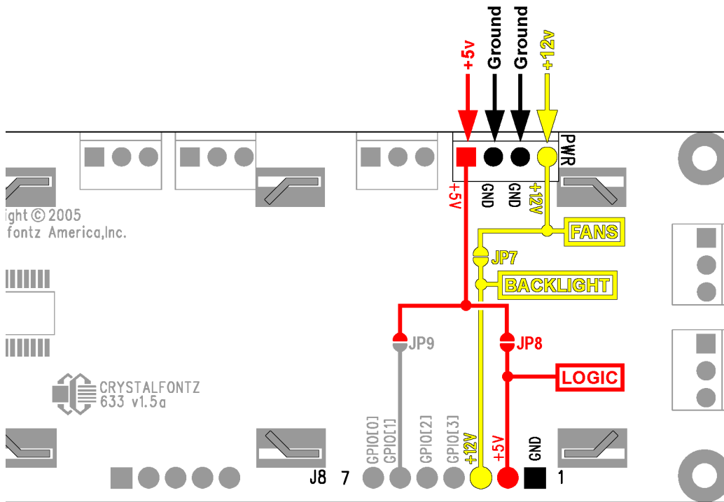
Figure 2. CFA-633 connection for standard "3 1/2 inch floppy" power supply cable
