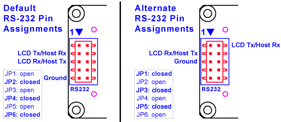
Figure 5. CFA-633 default and alternate pin assignments
