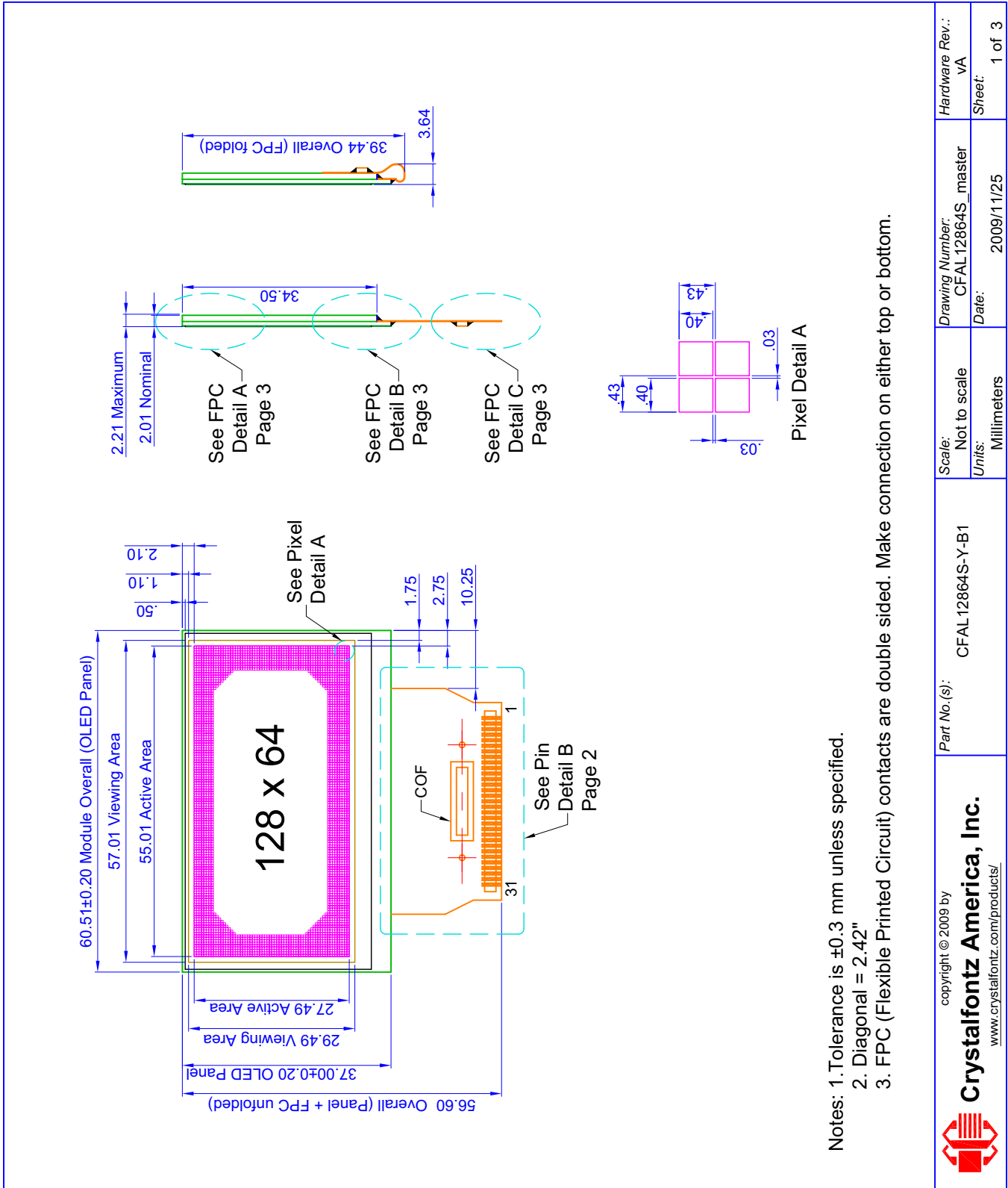
Figure 1. Module Outline Drawings (3 pages below)
