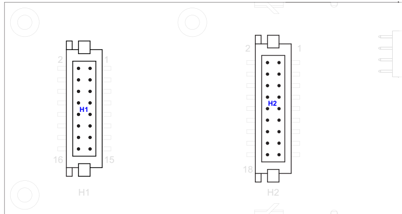
Figure 6. CFA635 Serial LCD Module Connectors H1 and H2
