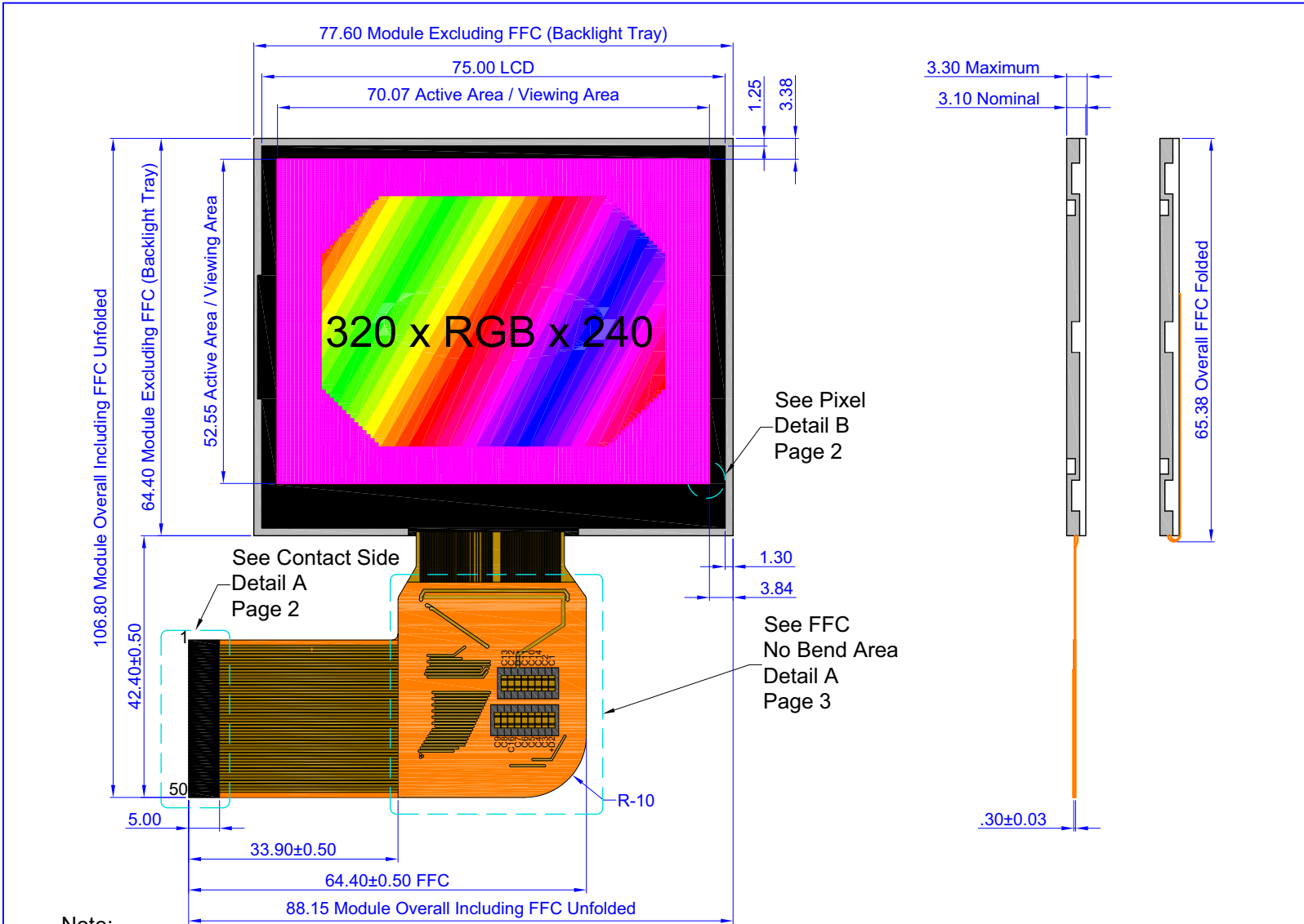
Figure 1. Module Outline Drawings (3 pages)
