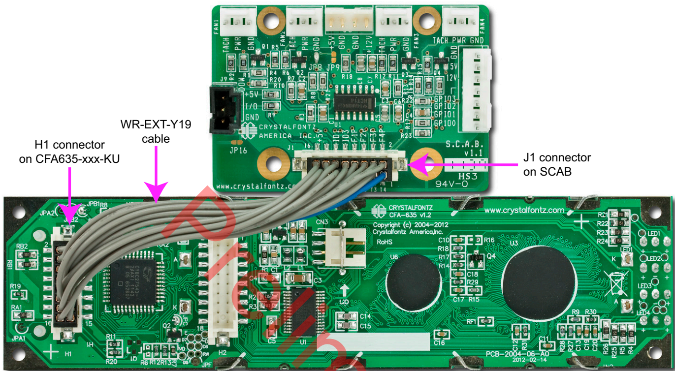
Figure 19. CFA635-xxx-KU Connected to Optional SCAB with WR-EXT-Y19 Cable
