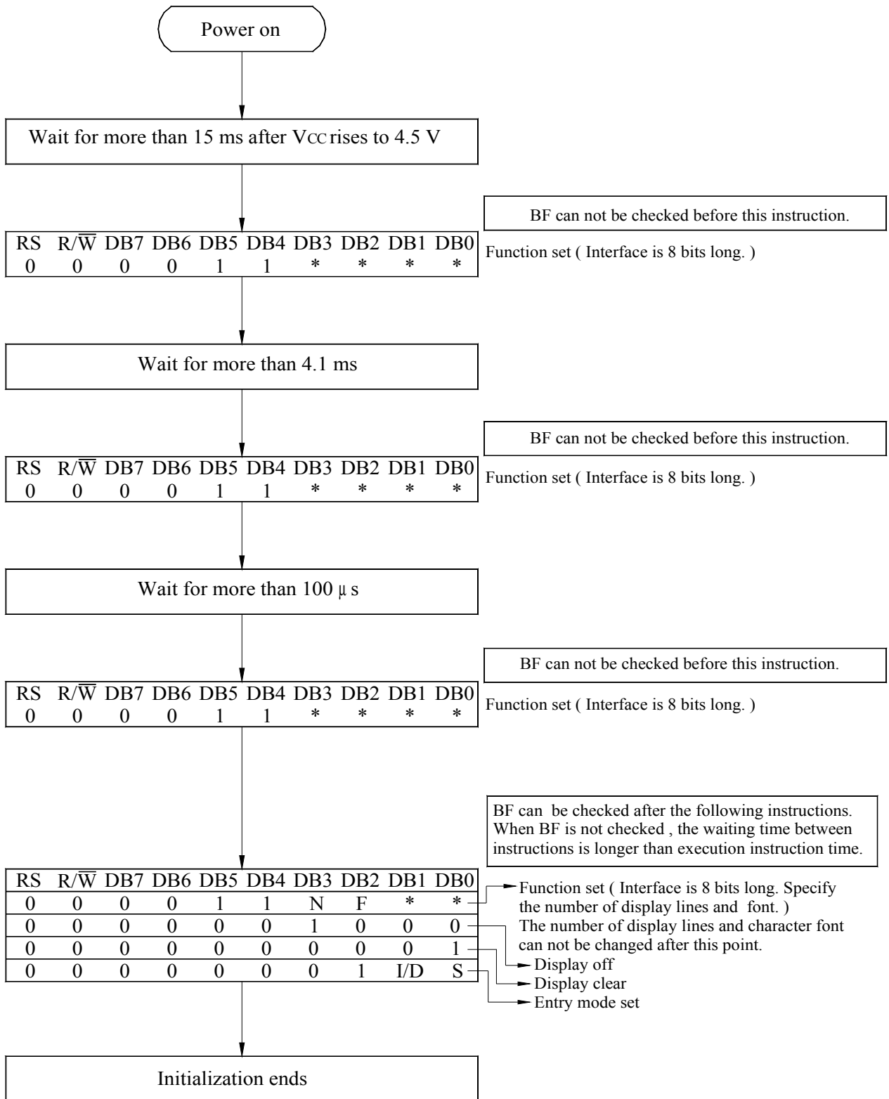
8-Bit Ineterface
