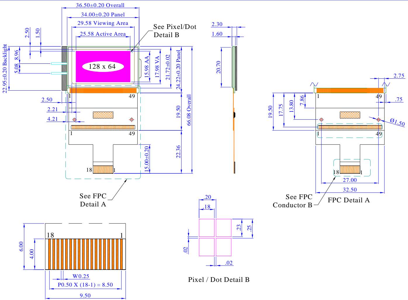
FPC Conductor Detail B
