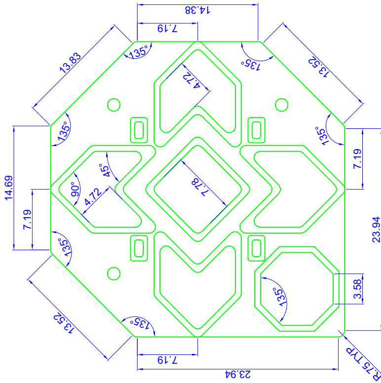
Keypad Detail
