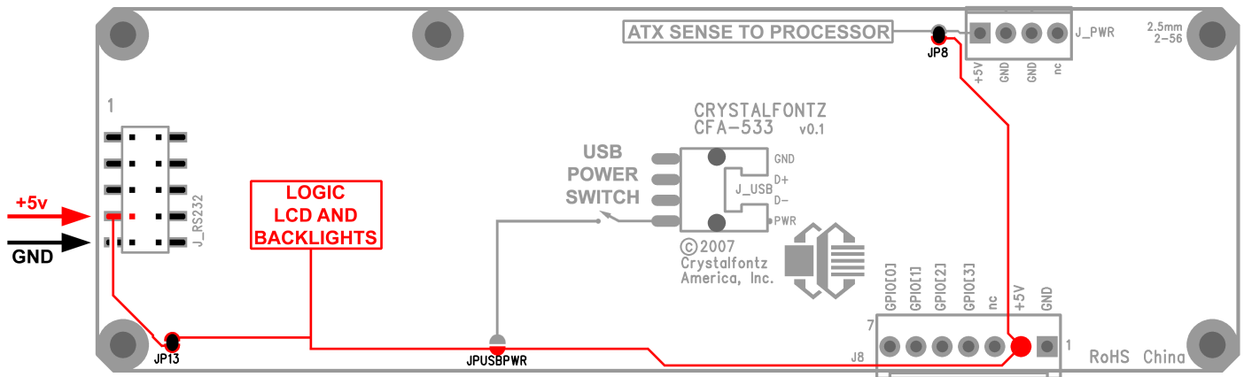
Figure 7. CFA533-TMI-KL RS-232 Power Connection
