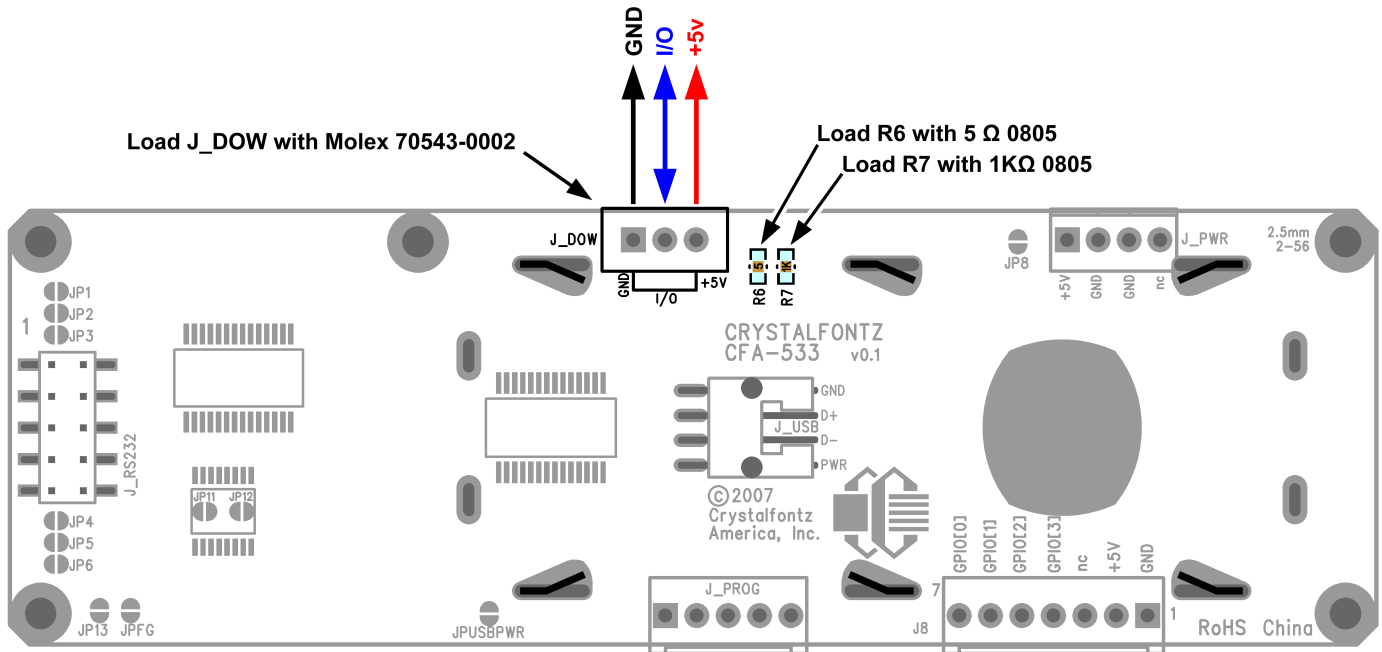
Figure 11. CFA533-TMI-KL Connection for Dallas Semiconductor 1-Wire (DOW) Devices
