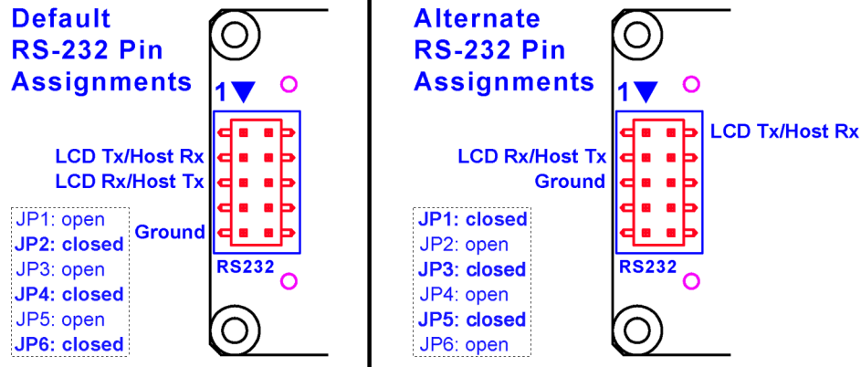
Figure 9. CFA533-TMI-KL Default and Alternate Pin Assignments
