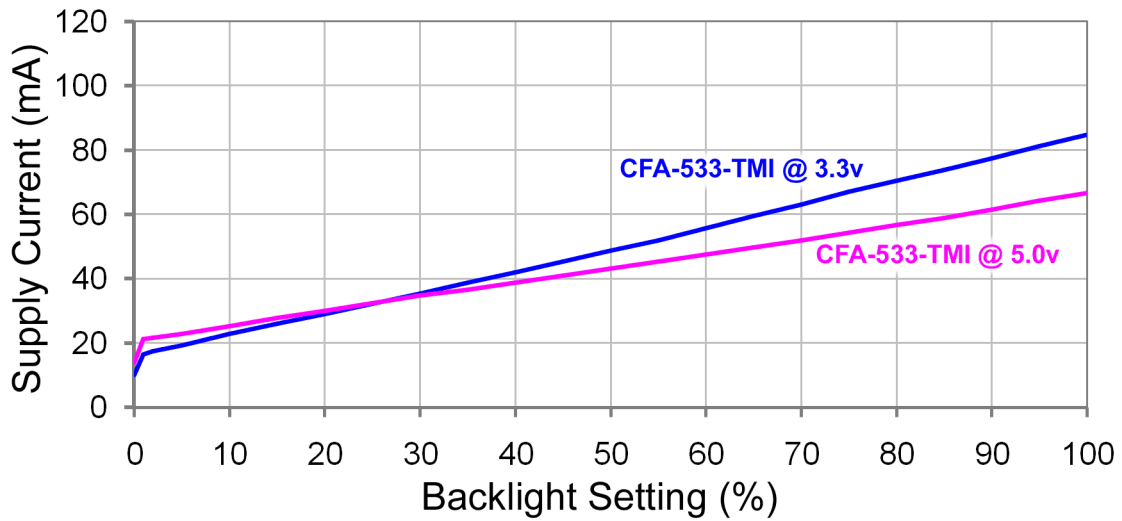
Figure 5. CFA533-TMI-KL Supply Current vs. Voltage and Backlight Setting
