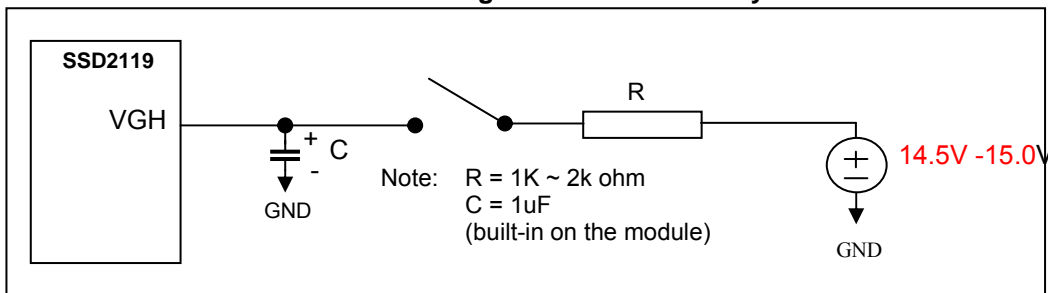
Figure 9-3: OTP circuitry
