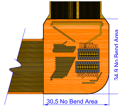
FFC No Bend Area Detail 'B'
