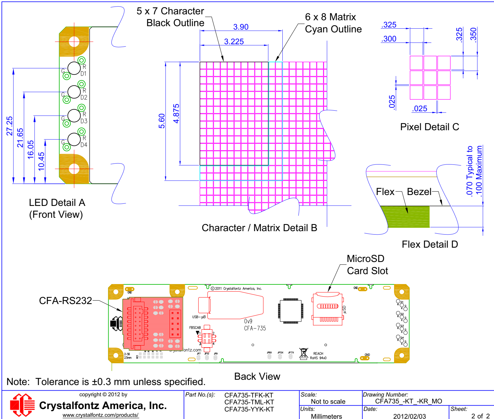
Figure 3. Module Outline Drawing Back View and Pixel Detail
