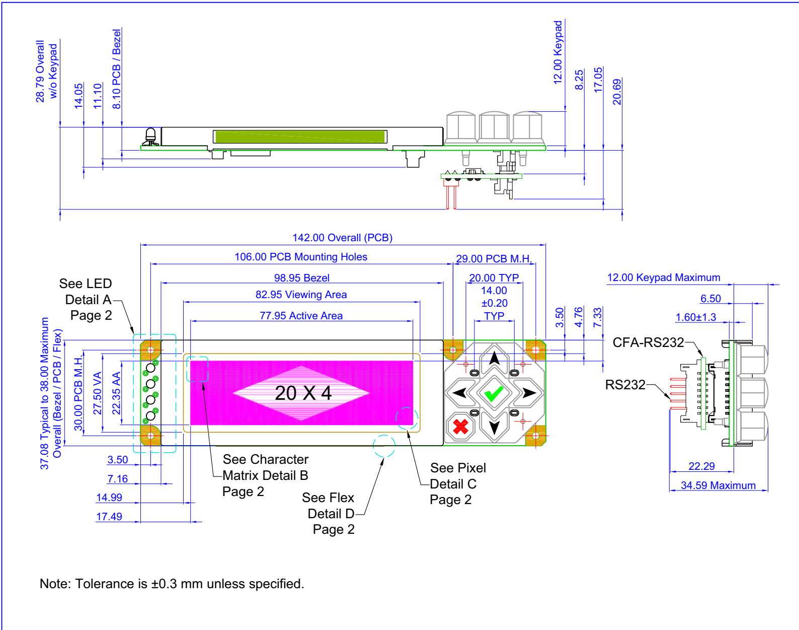
Figure 2. Module Outline Drawing Front and Side Views
