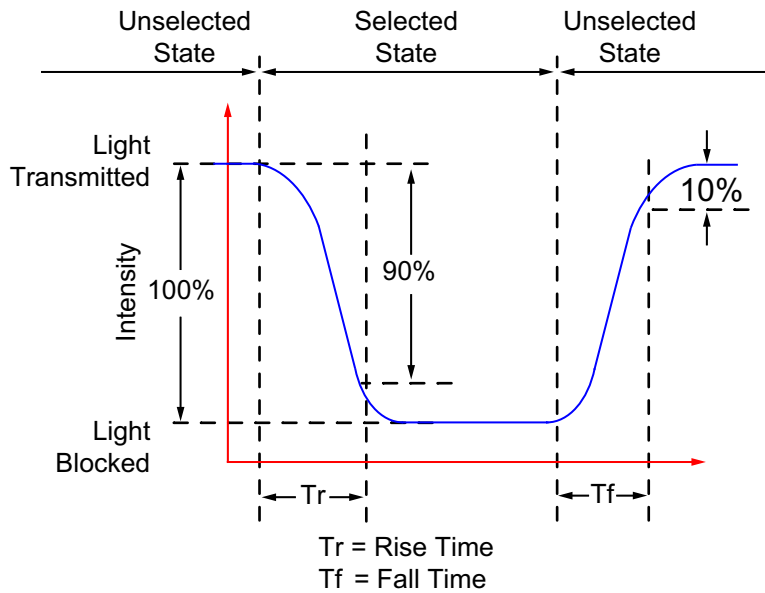
Figure 10. Definition of Response Time ( T_r , T_f ) (Positive Image)
