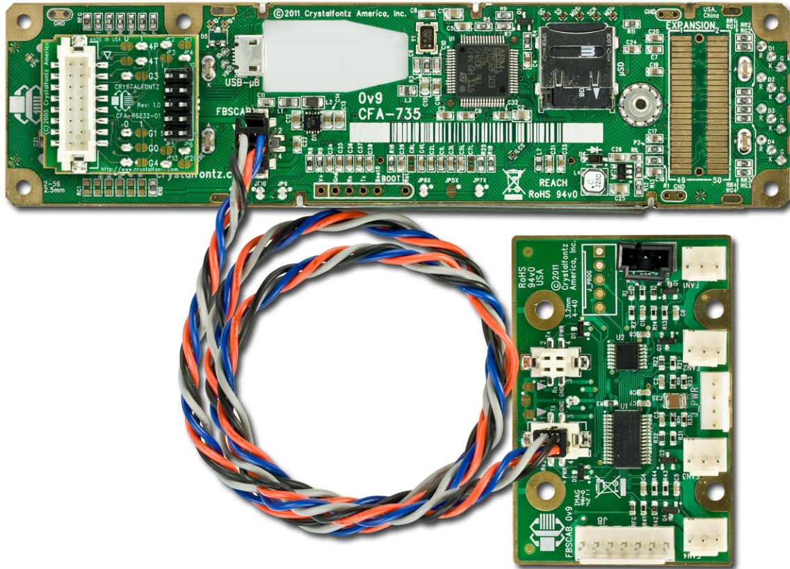
Figure 22. CFA735-xxx-KT Module Connected to Optional CFA-FBSCAB with WR-EXT-Y37 Cable
