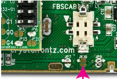
Leave JP10 open
