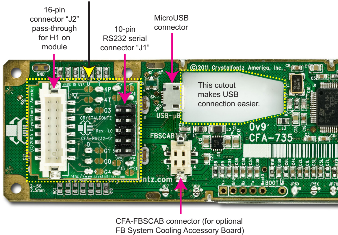
Figure 13. Location of Connectors
