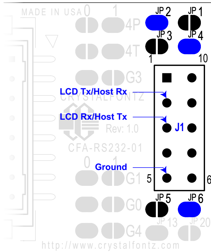
Figure 19. CFA-RS232 J1 Connector Default RS232 Pin Assignments
