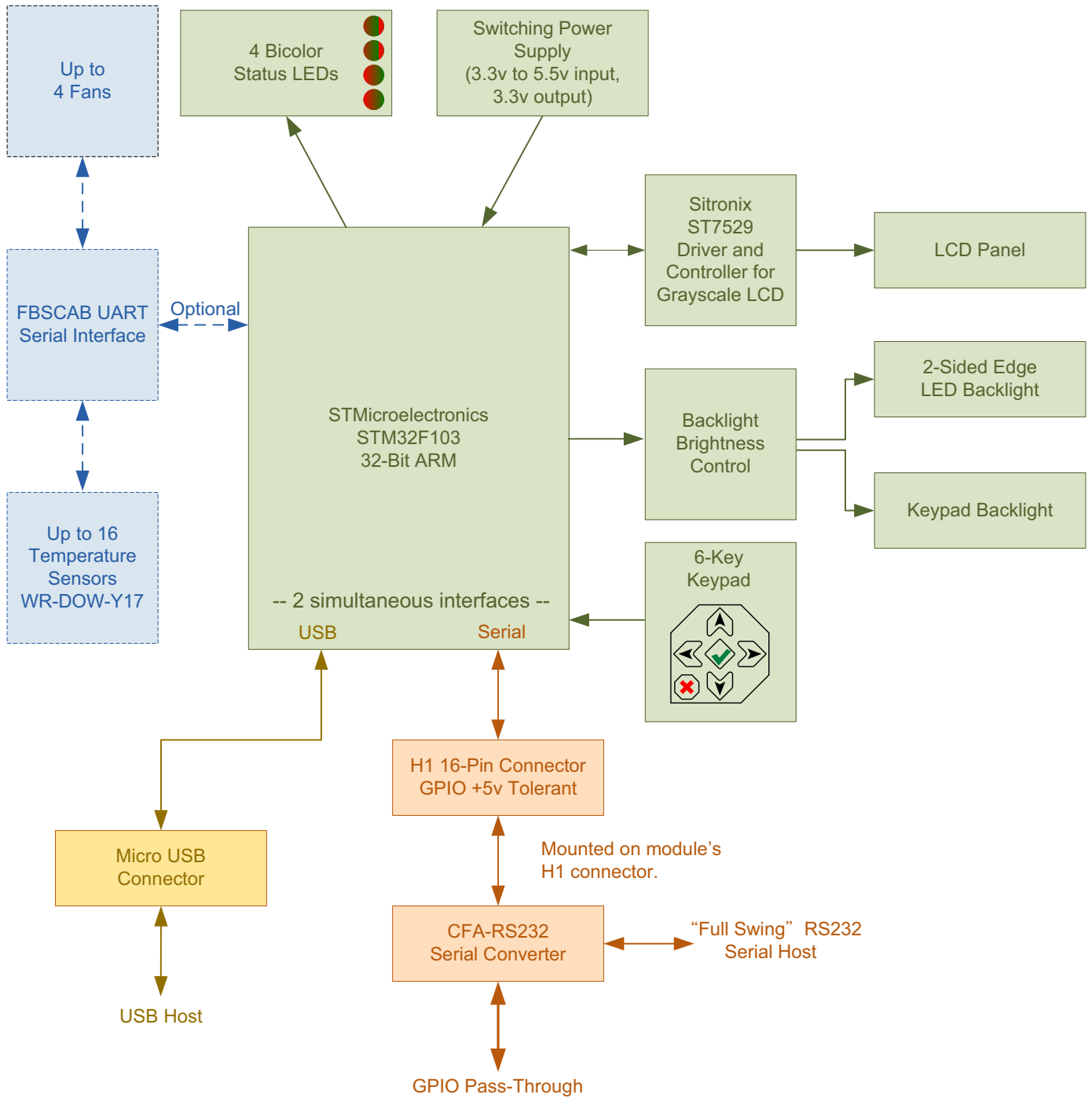
Figure 6. System Block Diagram
