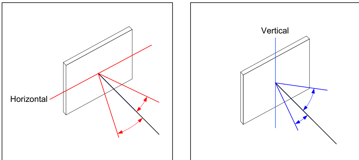
Figure 12. Definition of Horizontal and Vertical Viewing Angles (CR ≥ 2)
