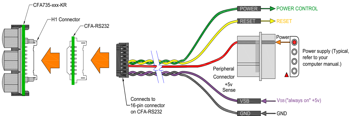
Figure 15. ATX Power Supply and Control Connections Using CrystalFontz WR-PWR-Y25 Cable
