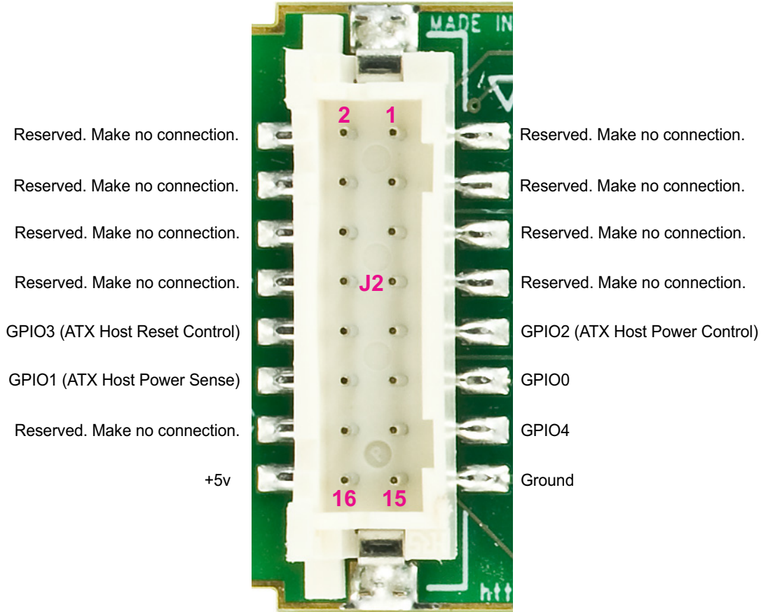
Figure 21. CFA-RS232 J2 Connector Pin Assignments
