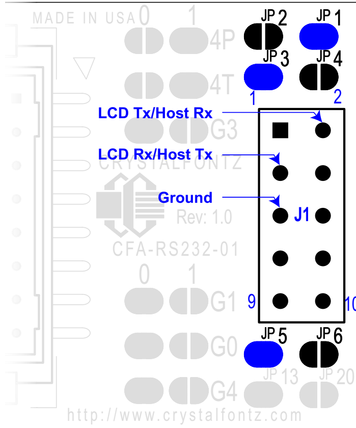
Figure 20. CFA-RS232 J1 Connector Alternate RS232 Pin Assignments
