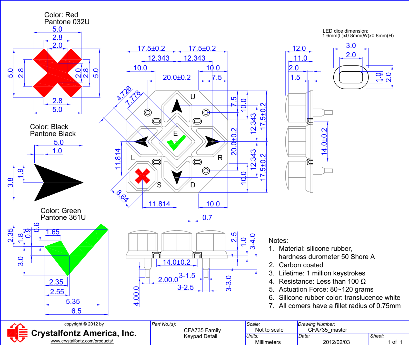
Figure 5: Keypad Detail Drawing
