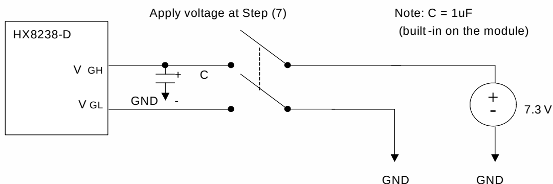
Figure 8. 2 OTP Programming Circuitry
