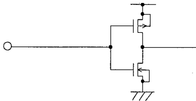
Input/Output Terminal Structure SIO Terminal
