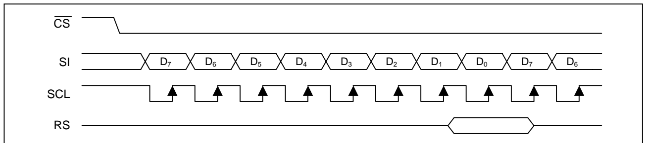
Fig. 8-1 4-line serial interface timing
