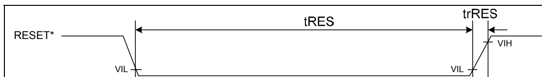
Figure 14-2 Reset Operation
