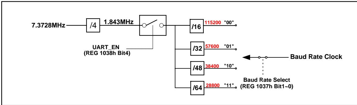
Figure 8-15 Baud Rate Clock Block Diagram
