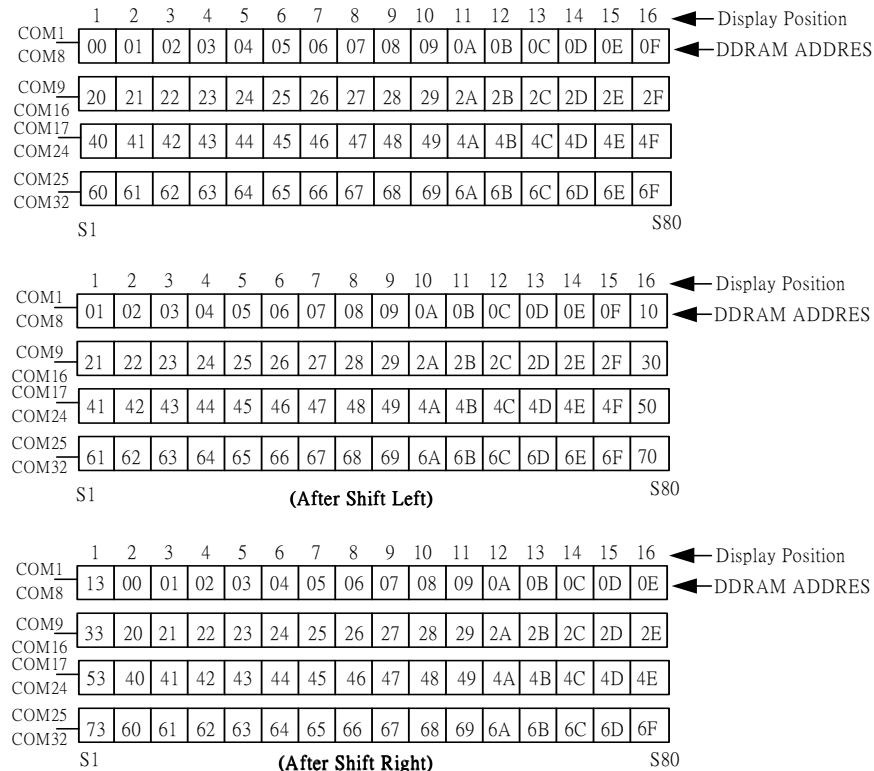
(Figure 3) 4 - line X 16ch. Display (5-dot Font Width)
