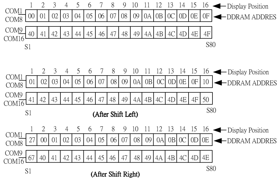
(Figure 2) 2 - line X 16ch. Display (5-dot Font Width)
