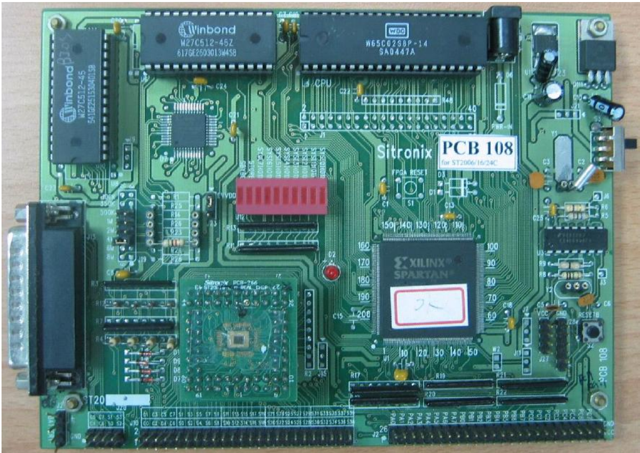
FIGURE 18-33: The PCB 108 of ST2016B EVB
