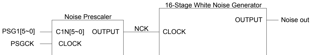
FIGURE 14-5 Noise Generator
