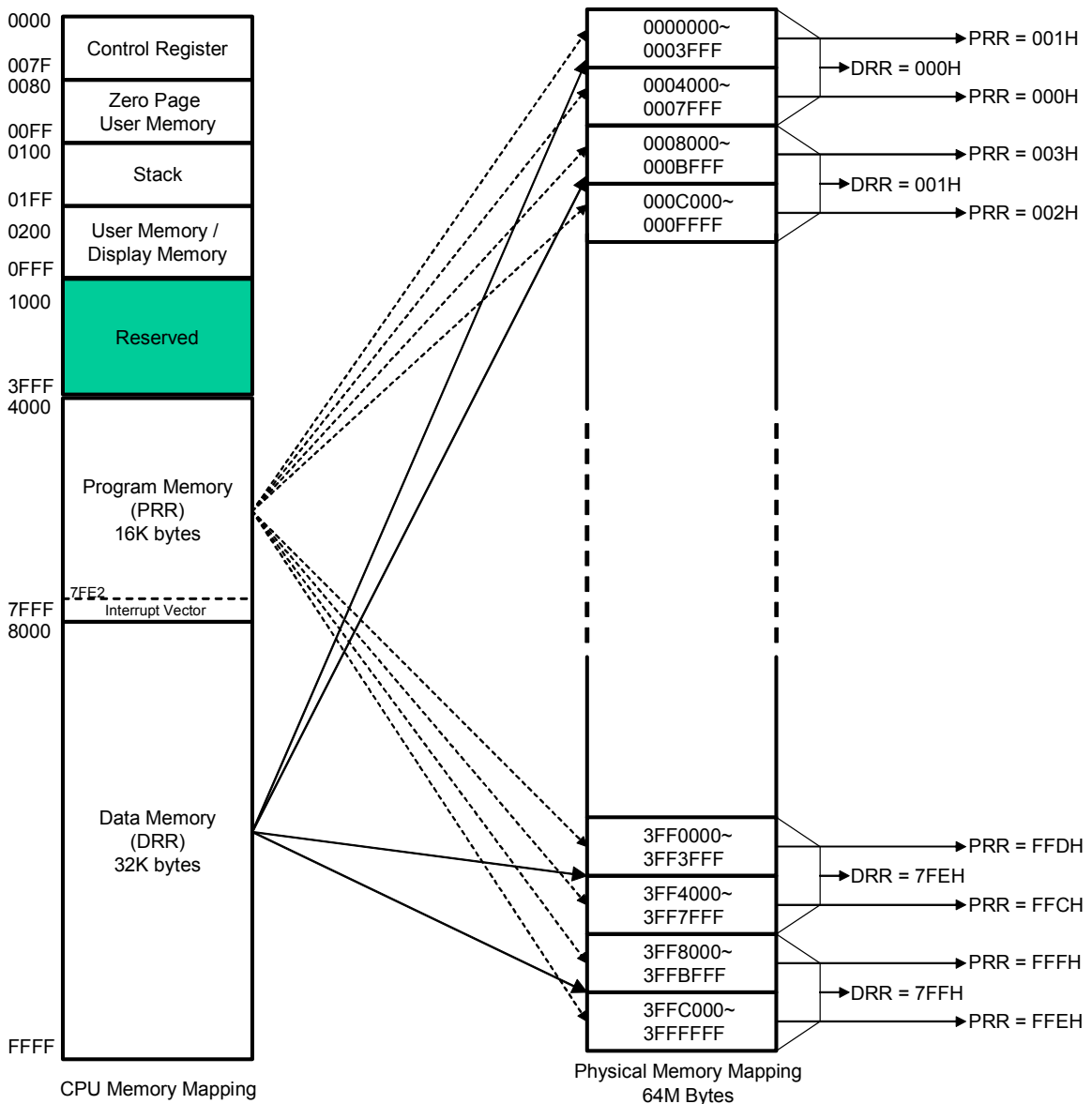
FIGURE 7-1 Memory Mapping
