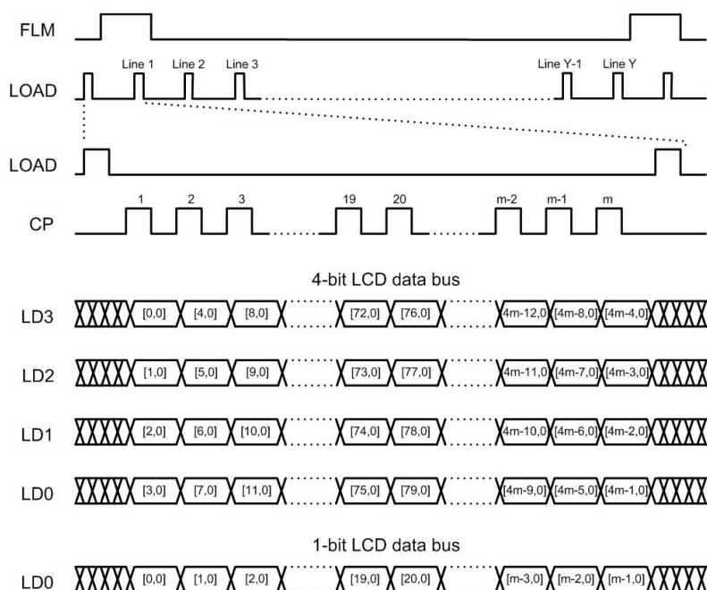
FIGURE 12-2 LCD Interface Timing for 1-/4-Bit Data
