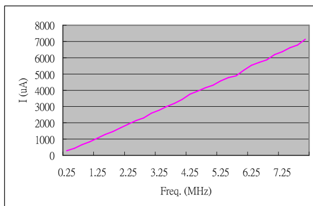
FIGURE 22-5 Operation Current as a function of OSCK
