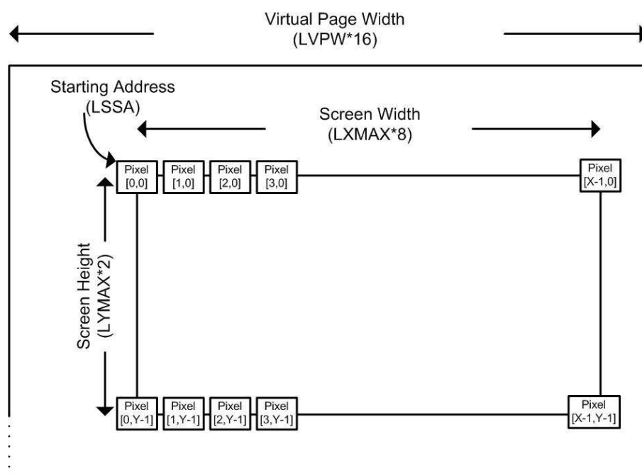
FIGURE 12-1 LCD Screen Format
