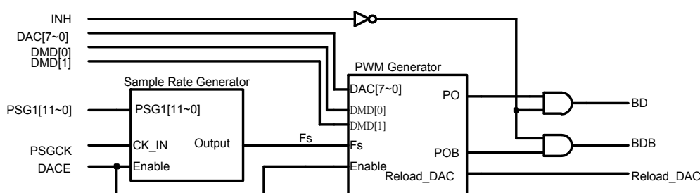
FIGURE 11-1 DAC Diagram
