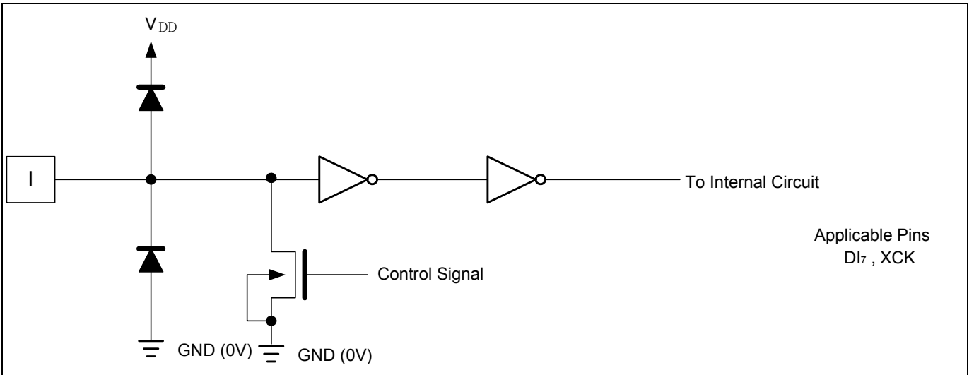
Figure 5-2 Input Circuit (2)
