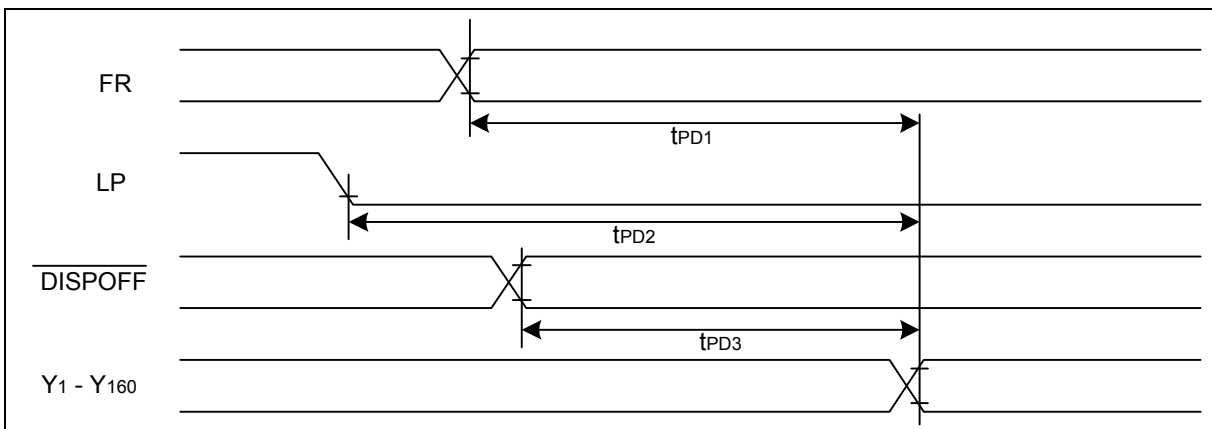
Figure 10-1 Timing Characteristics (3)
