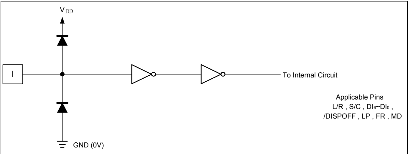
Figure 5-1 Input Circuit (1)
