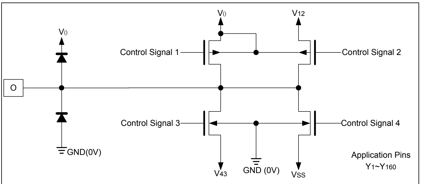
Figure 5-4 LCD Drive Output Circuit
