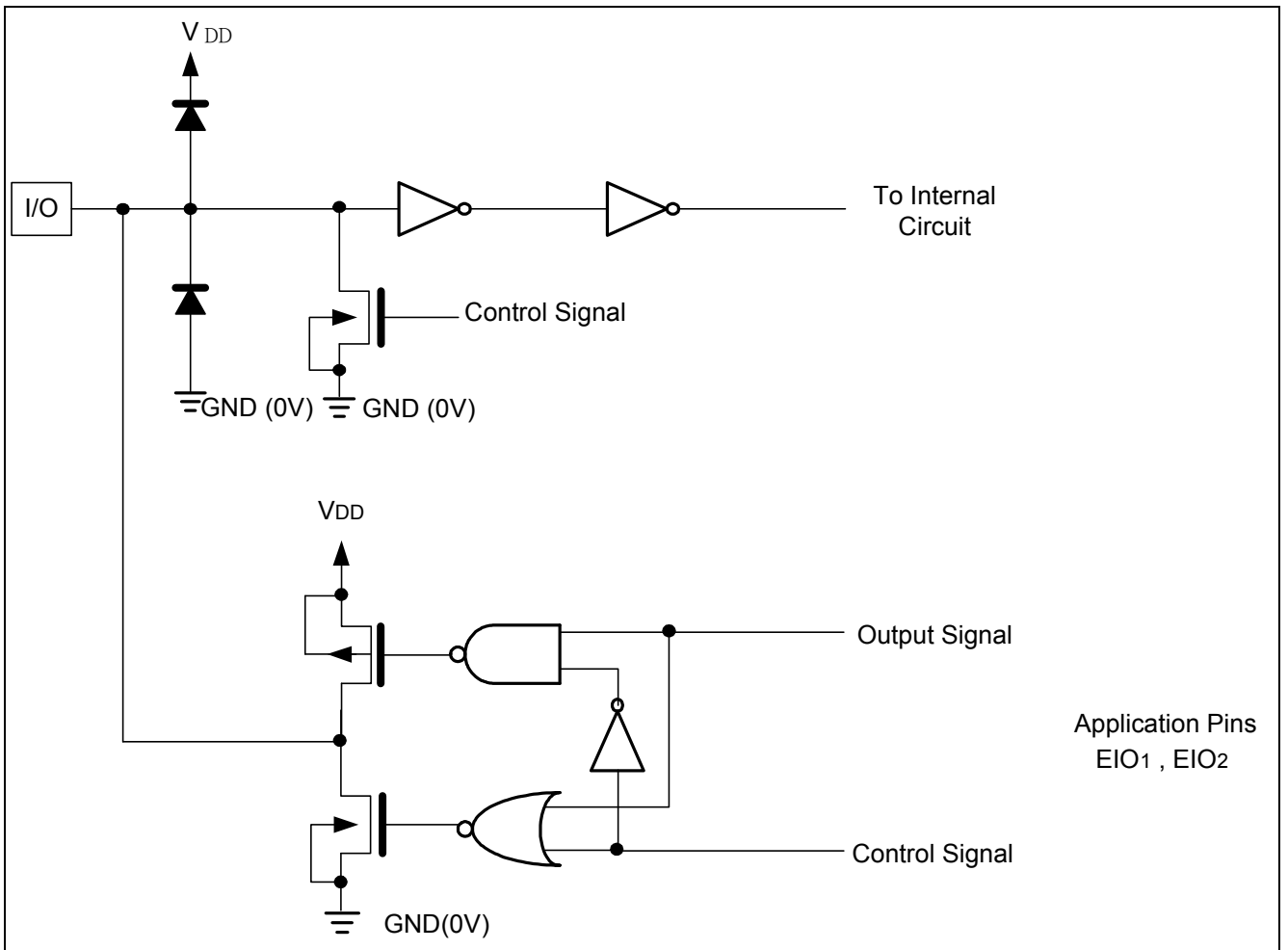
Figure 5-3 Input/Output Circuit
