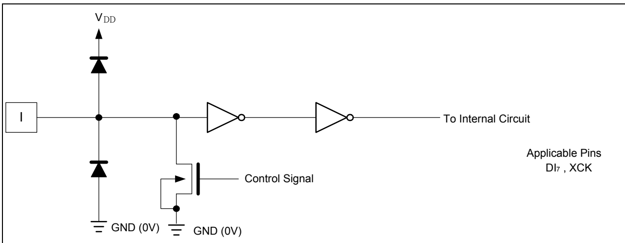
Figure 5-2 Input Circuit (2)
