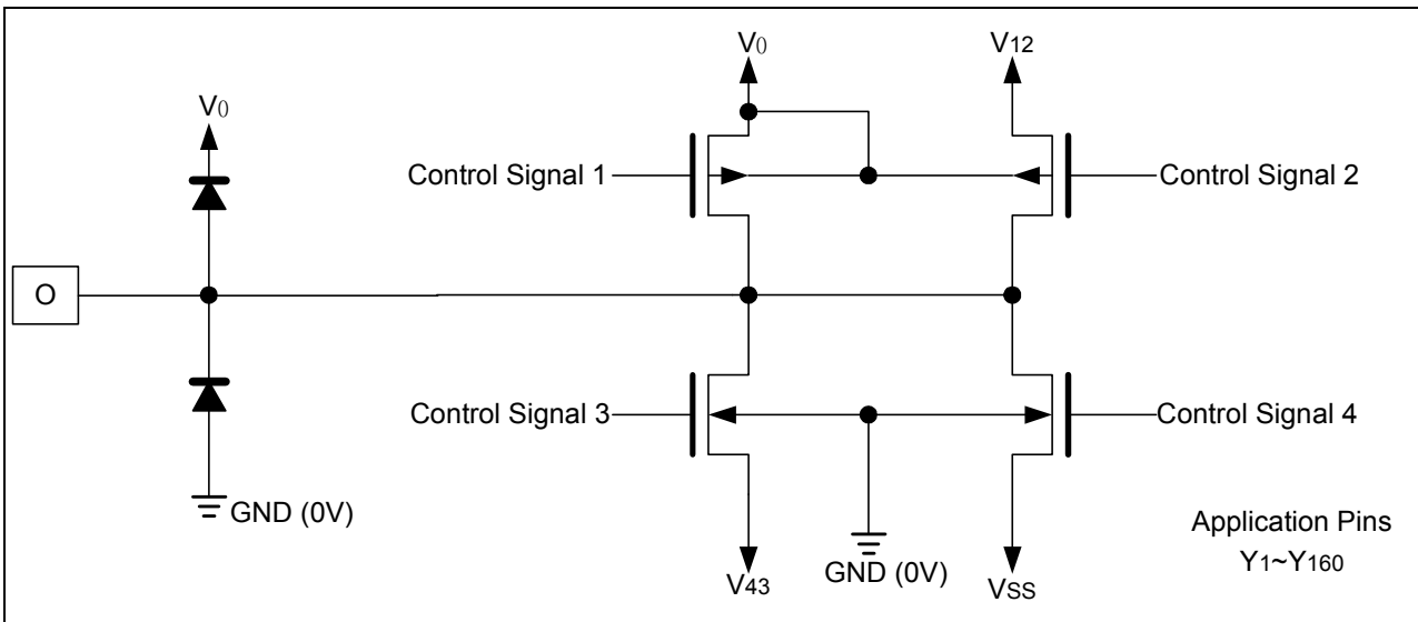
Figure 5-4 LCD Drive Output Circuit
