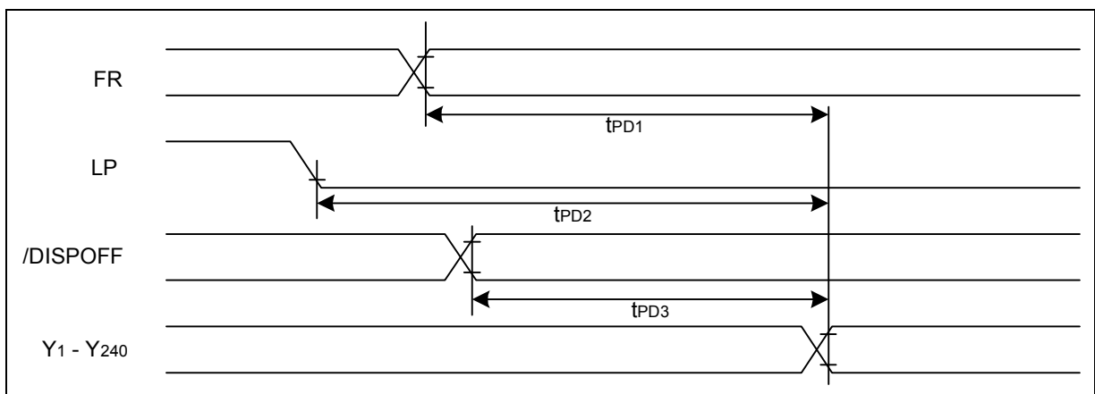
Figure 10-1 Timing Characteristics (3)
