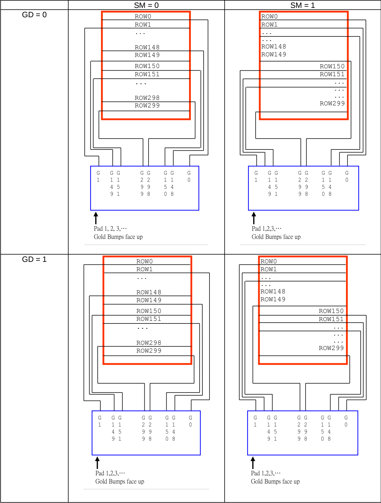
Figure 8-1: Output pin assignment on different Scan Mode Setting
