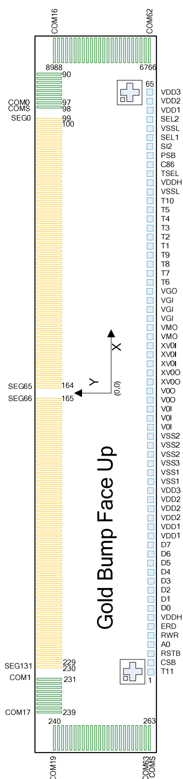
Figure 2 PAD Location
