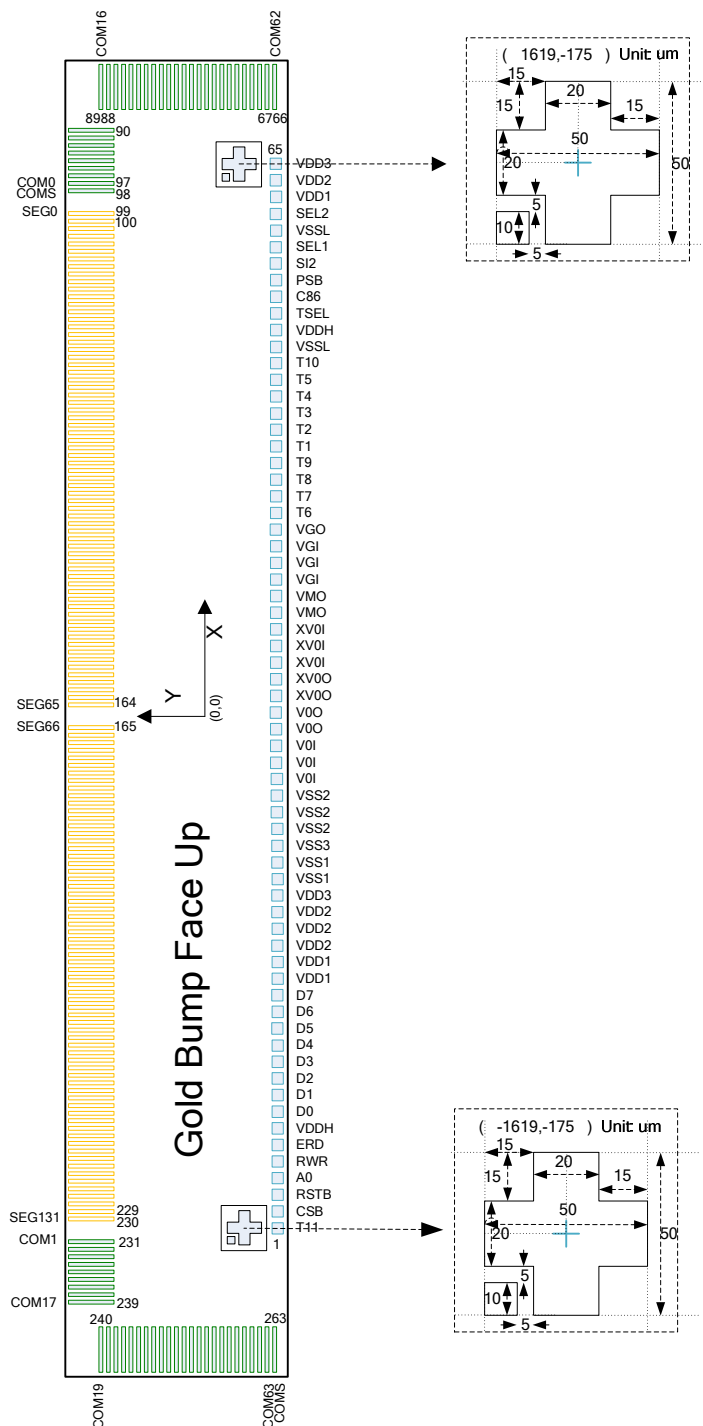
Figure 1 Chip Outline
