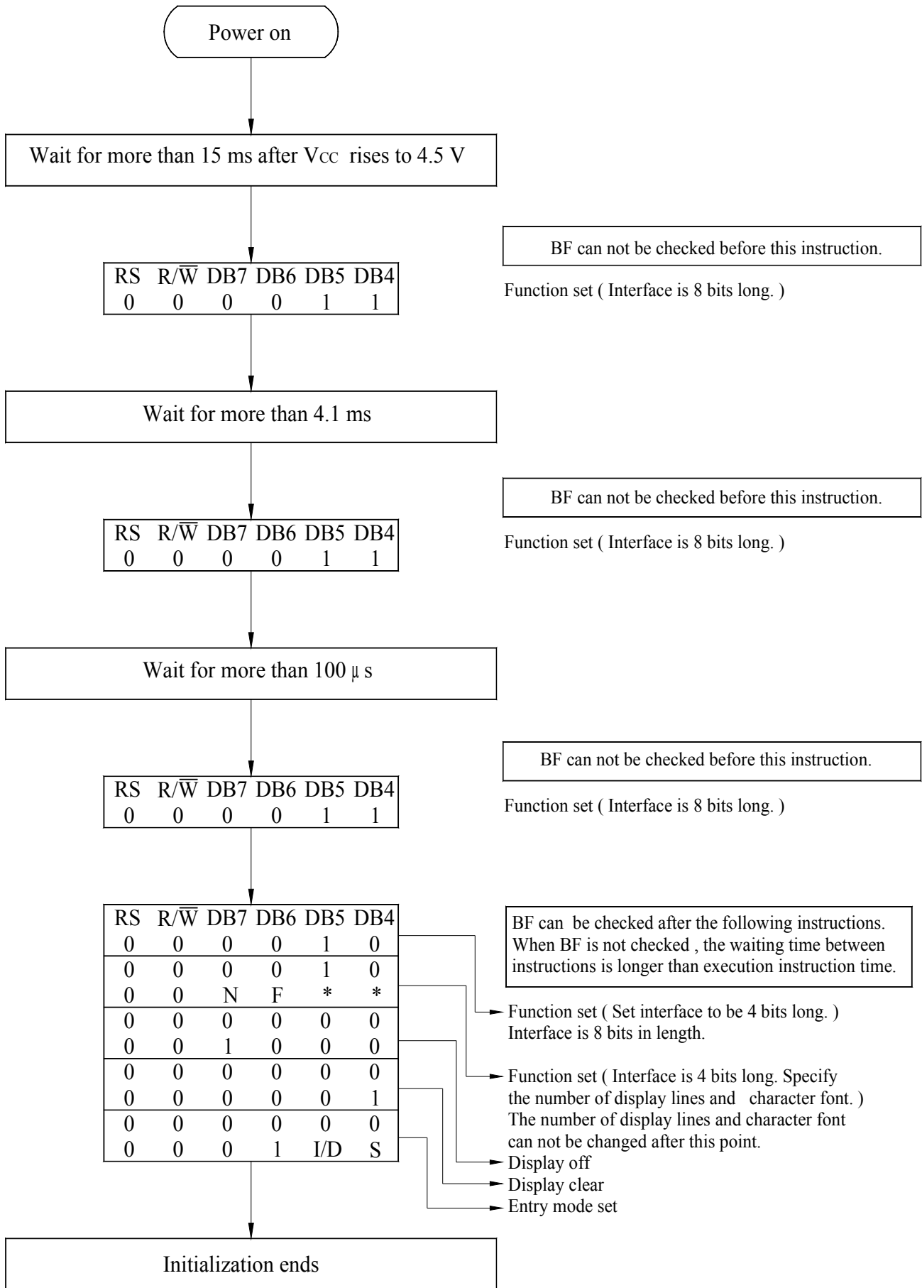
4-Bit Inerface
