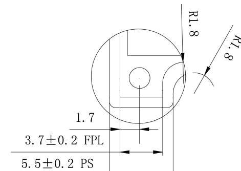
Detail B Scale 1/3
