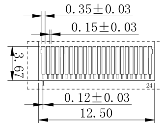
Detail A Scale 1/2.5
