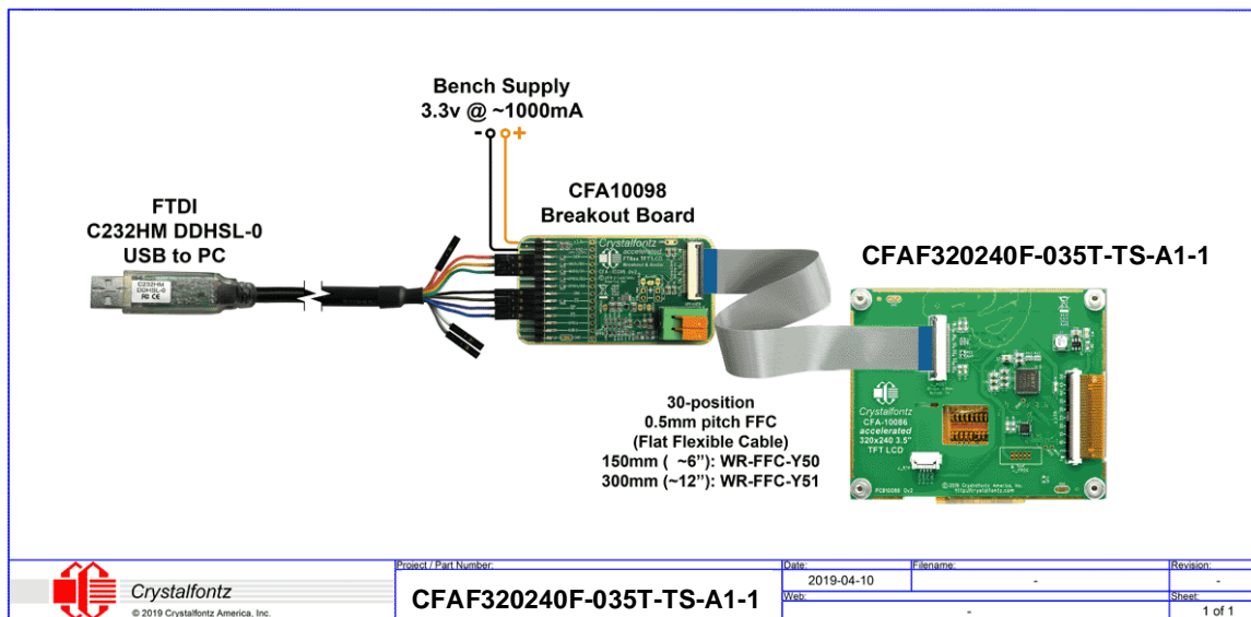
CFAF320240F-035T-TS-A1-1- CFA10098 - USB to PC
