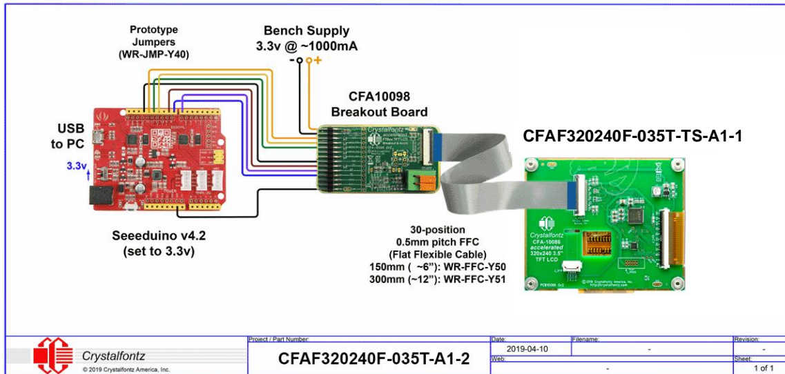
A1-2 Series comprising: CFAF320240F-035T-TS-A1- CFA10098 – Seedeuino
