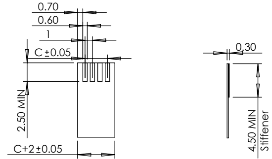
Recommended FFC/FPC
