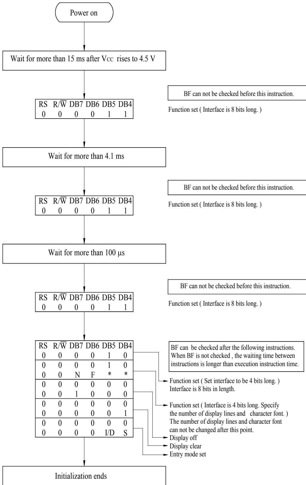
4-Bit Ineterface
